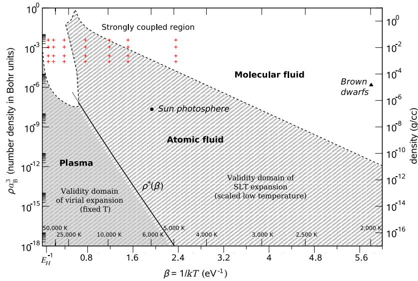
Figure 1. Validity domain of truncated SLT equation of state. Crosses indicate state points where PIMC simulation results are available [13].
